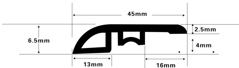
Reducer
