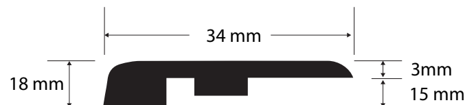
End-cap
