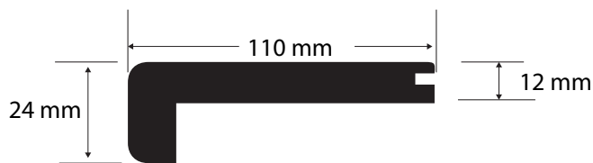
Flush Square Stairnose
