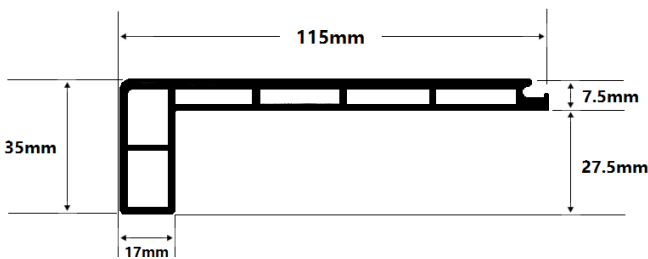
Flush square stairnose
