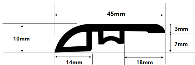
Reducer
