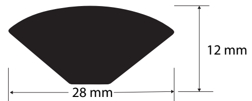
Quarter Round
