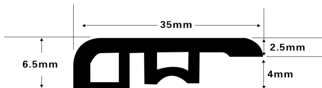
End-cap
