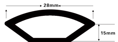
Quarter round
