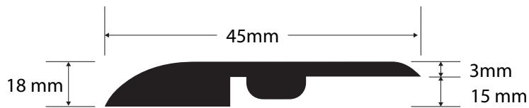
Reducer
